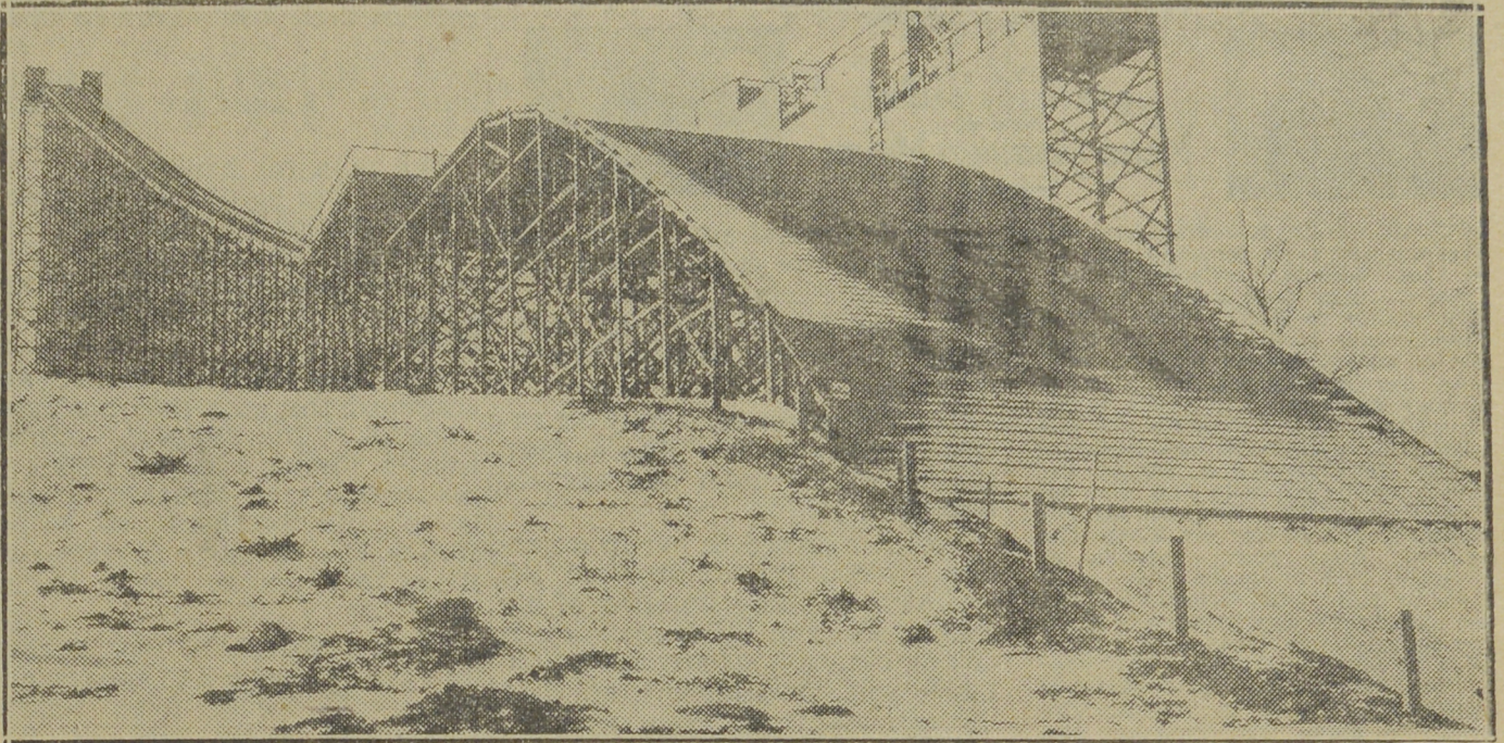
A view of the completed trestle ski-jump, the longest in the world, which has just been completed at Littleton, Mass., by the Eastern Professional Ski Association. The jump is over 600 feet from top to bottom, with a 60-foot gap in the centre, to furnish plenty of thrills to spectators and skiers alike. The jump cost $20,000
