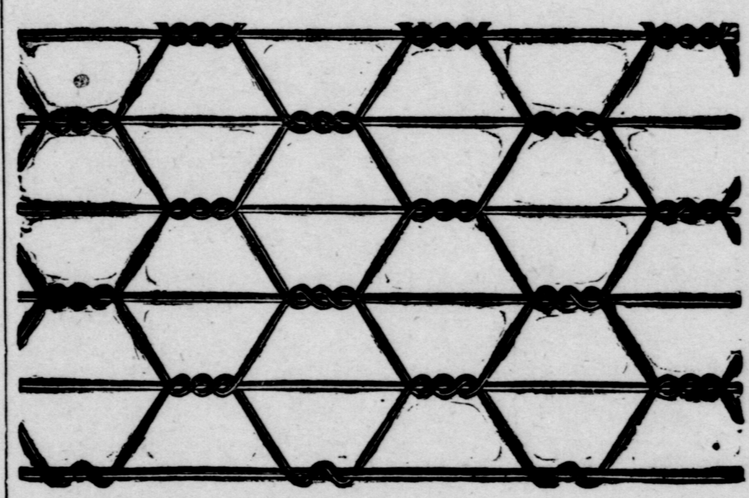
The above cut correctly represents the twist and manner in which the straight wires go through the mesh or diamond in the fence, made on the Kitzelman Woven Wire Fence Machine.
