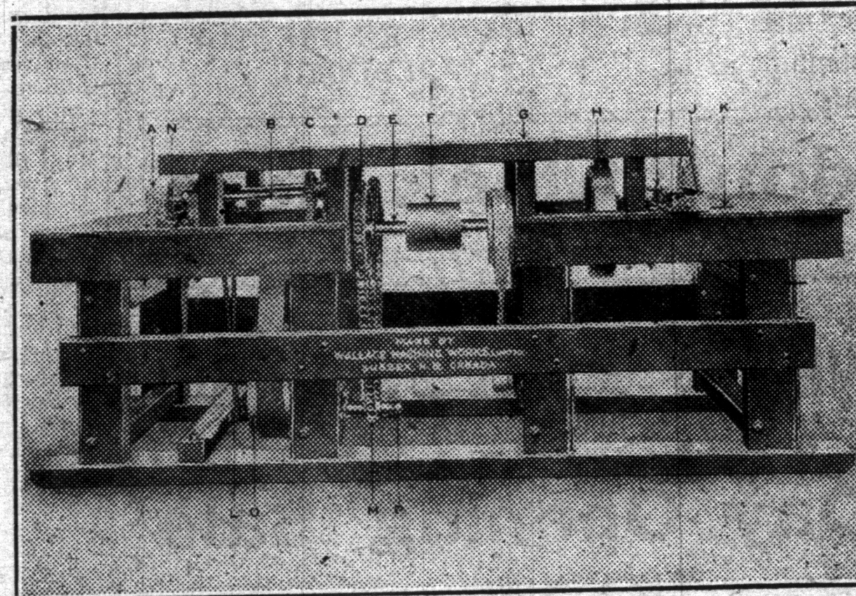
The Famous Patented Wallace Portable Lath and Bolter Machine.
