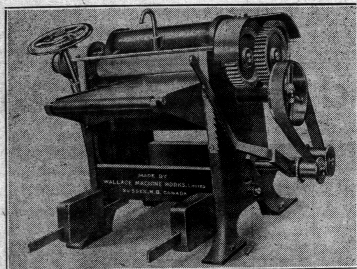
The Portable Mill Planer with Countershaft Attached.
