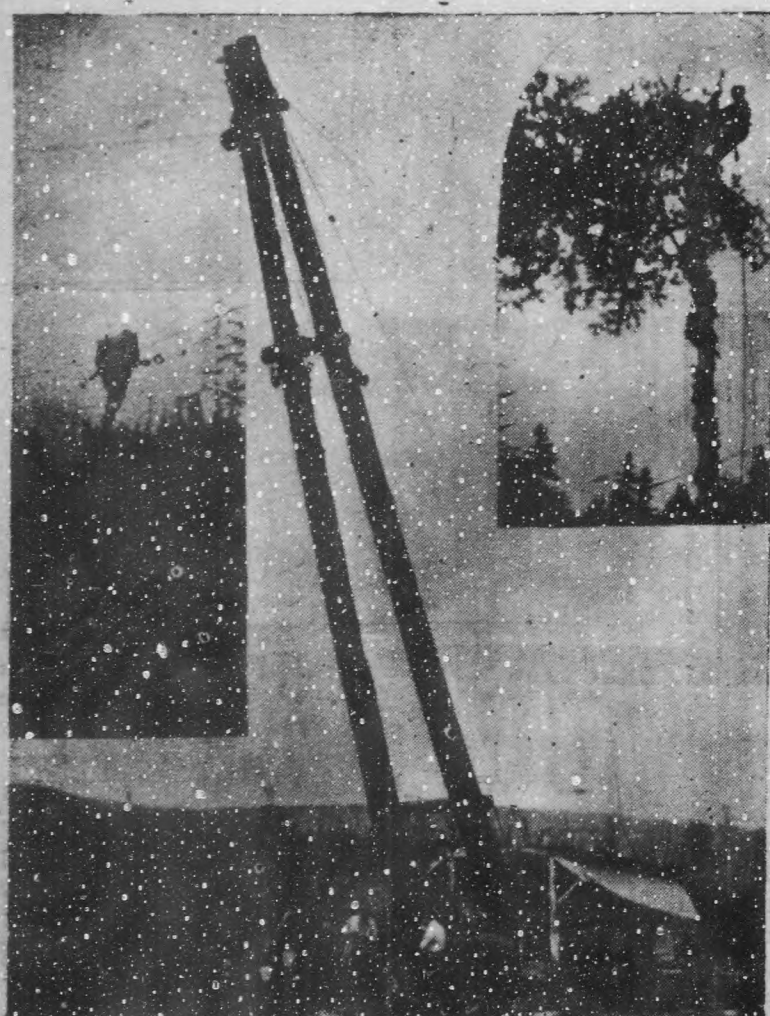
Picture of "A" frame showing, at top, sky-line, and, immediately below, main-line. At centre, on cross-piece, is the haulback; the other lines are the guy-wires. Left: carriage, showing pulleys, position of cables, and chokers attached to logs. Right: topping a birch for a spar-tree.
