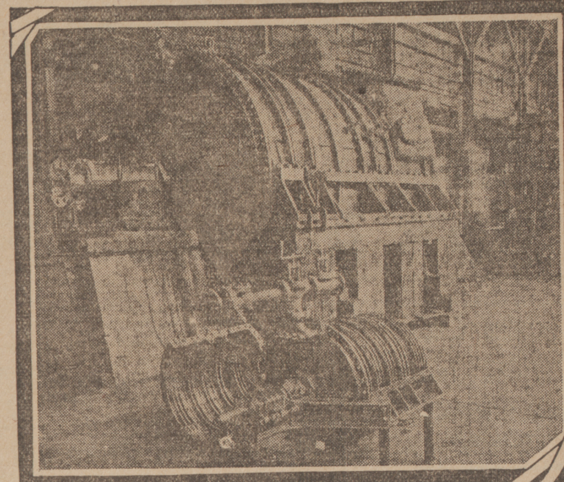
AT 8,000 HORSEPOWER AND A 250 TON WEIGHT MARINE TURBINE, THE FIRST AMERICAN -BUILT OCEAN-BOILING TURBINE
