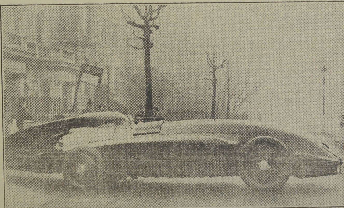
A side view of the "Flying Spray," a new racing car in which Captain G. E. T. Eyston hopes to set a new world's record for diesel-engined cars on Pendine Sands, England. This racing car, shaped very much after the style of Sir Malcolm Campbell's famous "Bluebird," is driven by heavy diesel engines of a new type.
